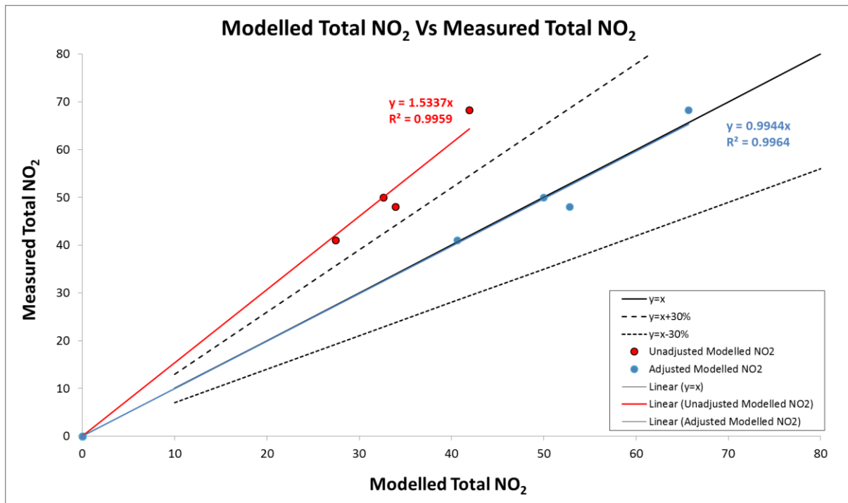
Figure 6: Comparison of modelled NO 2 before and after model verification
