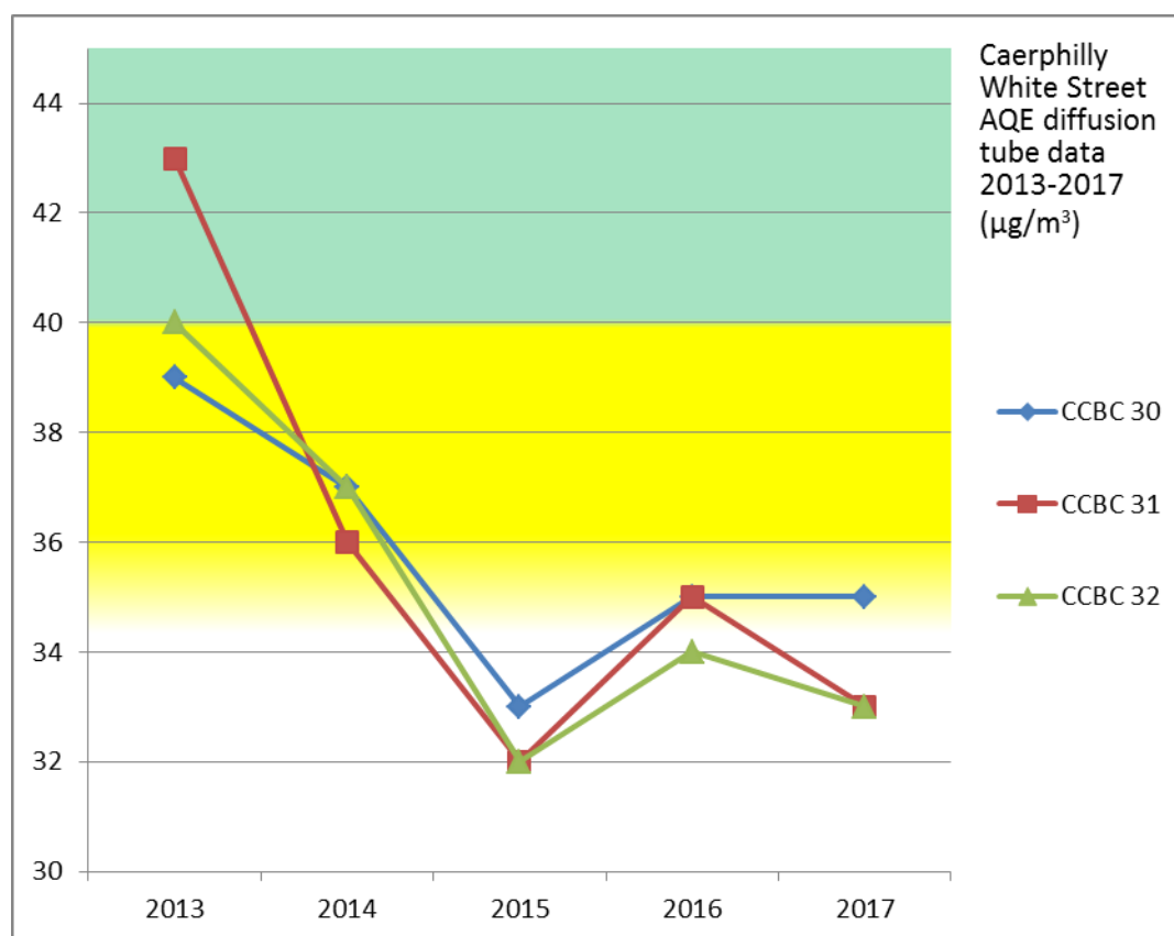
Figure 6 – Chart of Caerphilly Air Quality Enclosure Co-Located Diffusion Tube results 2013-2017
