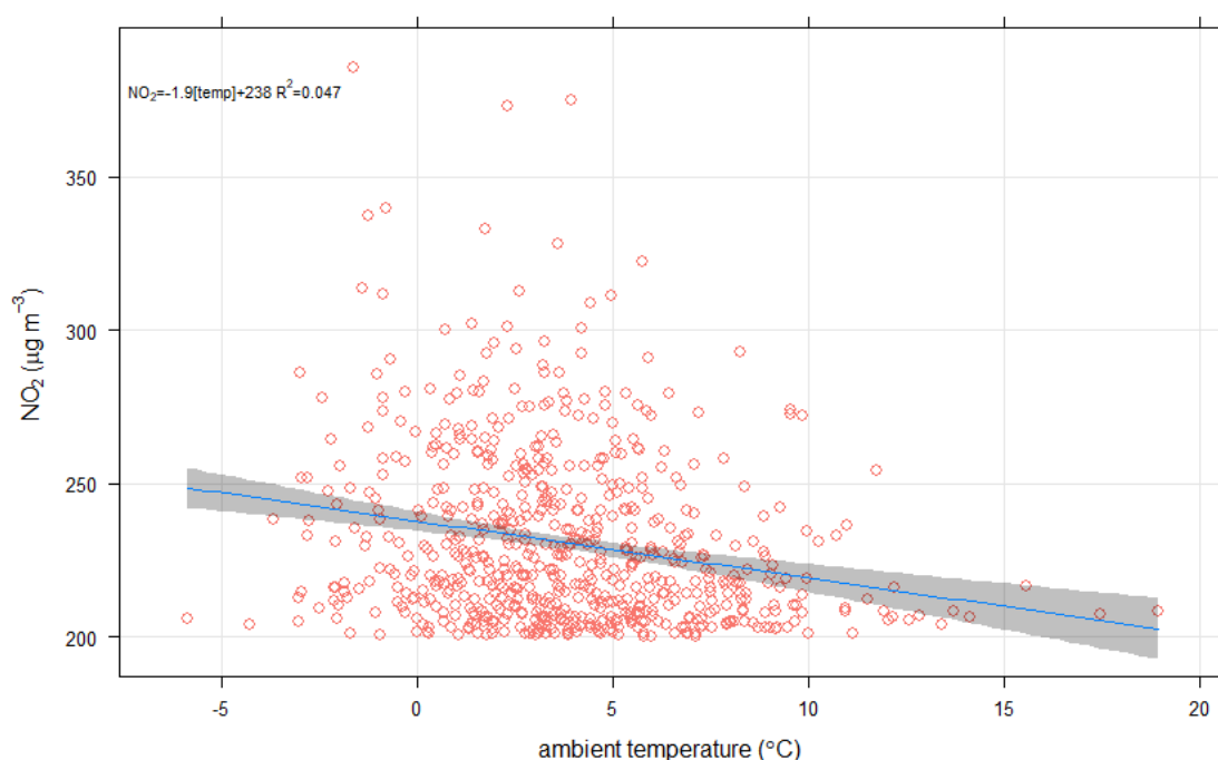
Figure 9: Scatterplot showing relationship between exceedances of the hourly objective and temperature
